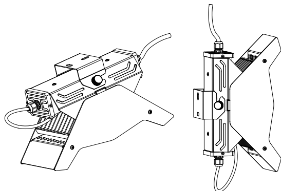
Universal mounting plate
