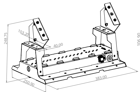
Tilted bracket kit
