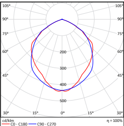
Symmetric optic
