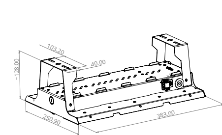
Rod Mount (optional)
